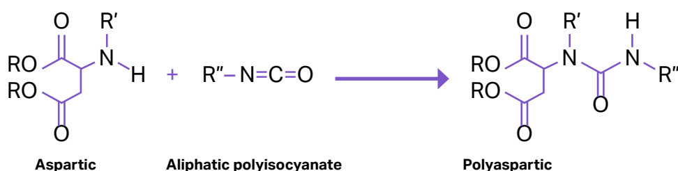
Fig. 7: Reaction of aspartics with aliphatic polyisocyanate to give polyaspartics
