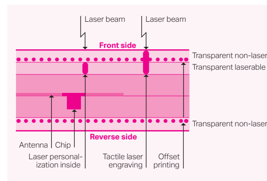
Structure of a Makrofol® ID card
