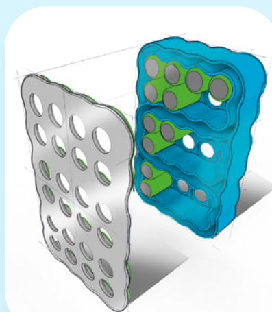
Battery pack with optimized cooling channels.
