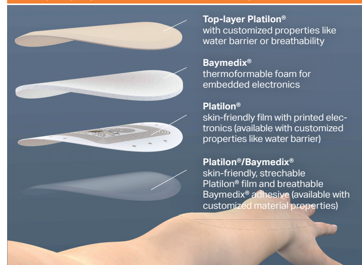
Exemplary layer structure for wearable patches
