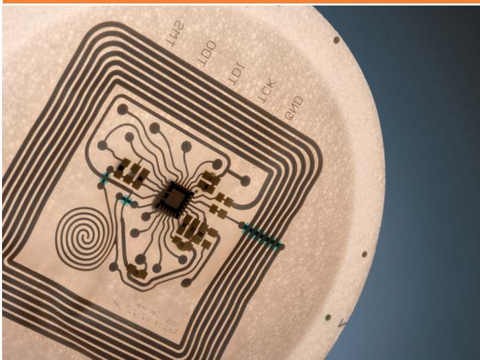
Exemplary Platilon® film with printed electronics
